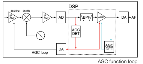
AGC function loop
